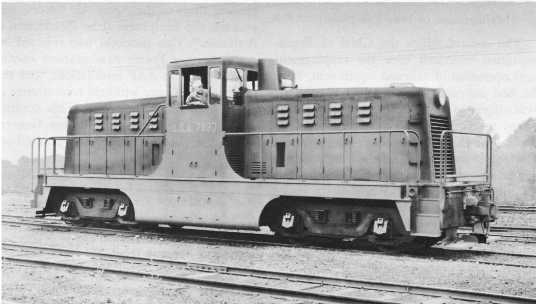
LOCOMOTIVES FOR UTILITY RAILROADS. Prewar 20-ton gasoline switcher, used for light work (top). An 80-ton diesel-electric, introduced during the war for the heavier switching jobs at Army installations (bottom).
