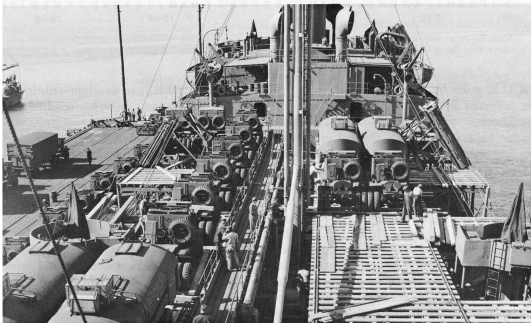
CRATED AND UNCRATED EQUIPMENT STOWED ON DECK. All available deck areas were utilized in order to achieve the maximum cargo lift.
