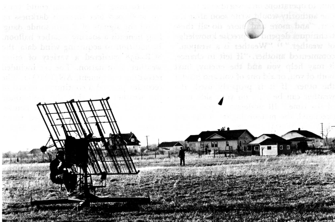
SCR-658 TRAINED ON RADIOSONDE AN/AMT-2 AT LAUNCHING
