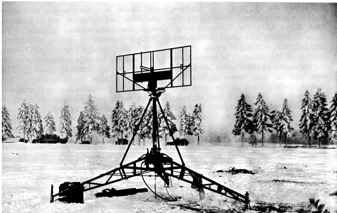
IFF ANTENNA USED BY THE 217TH ANTIAIRCRAFT BATTALION NEAR BASTOGNE
