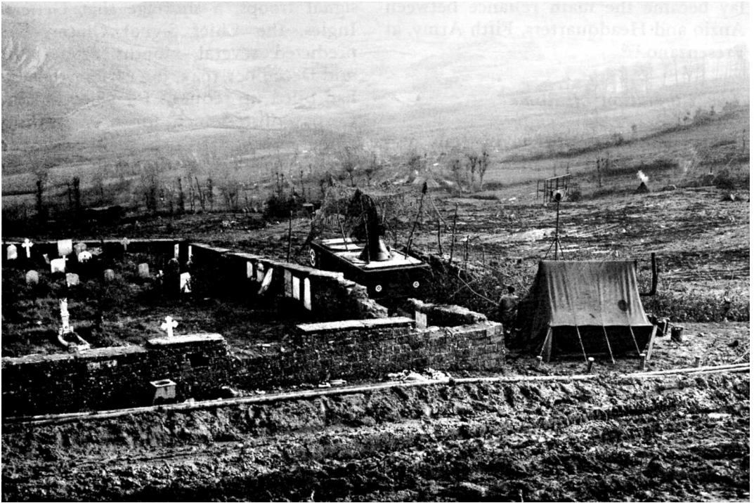
CAMOUFLAGED SCR-584 RADAR AND IFF (RIGHT) BESIDE A CEMETERY IN ITALY
