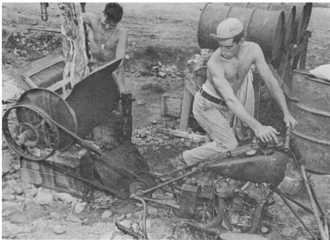
MAKESHIFT WASHING MACHINE built from a steel drum and a motorcycle, Port Moresby, New Guinea.
