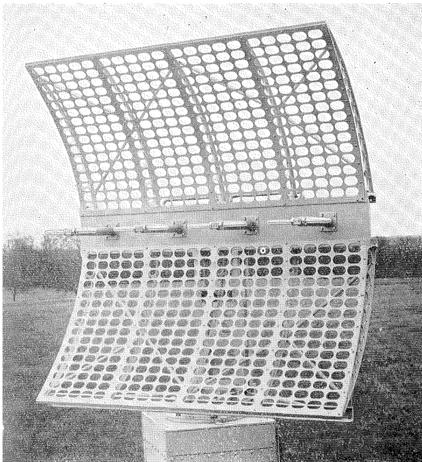
Fig. 3—CXAS—Antenna
