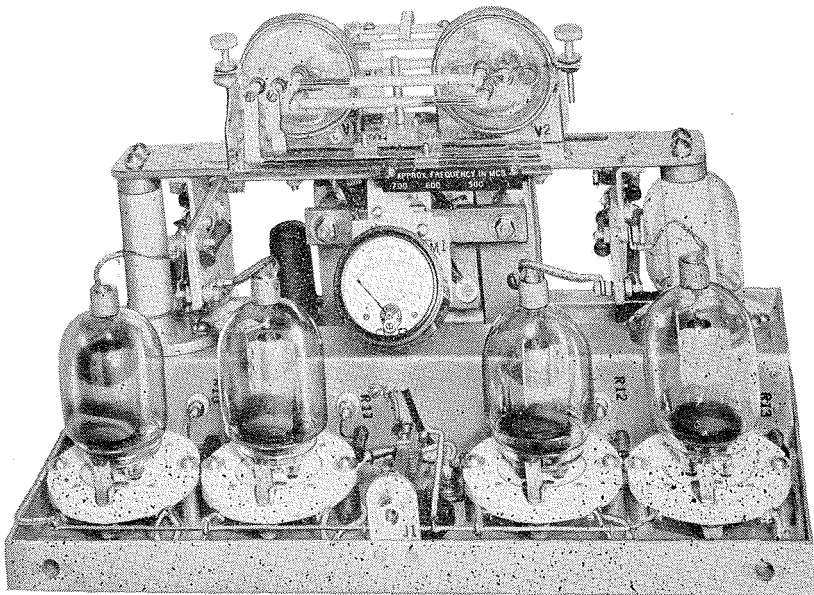
Fig. 13—CXAS—Transmitter
