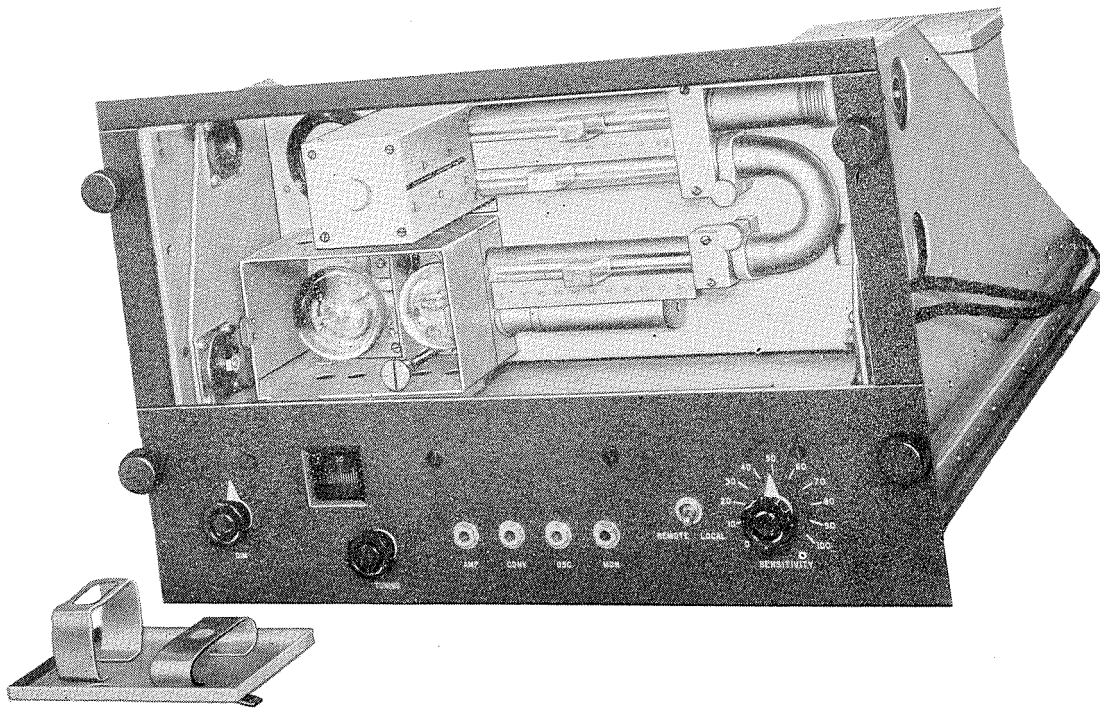
Fig. 11—CXAS—Receiver
