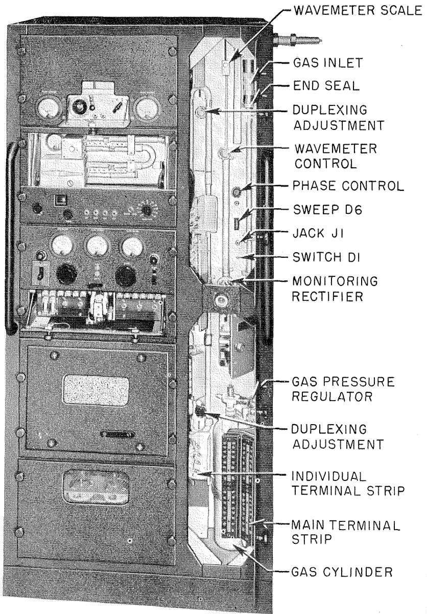
Fig. 9—CXAS—Main unit
