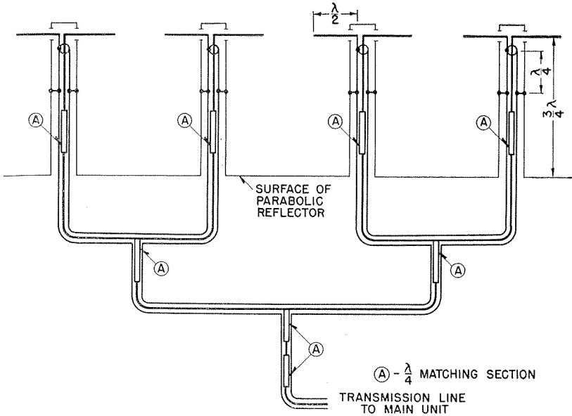
Fig. 5—CXAS—Antenna schematic
